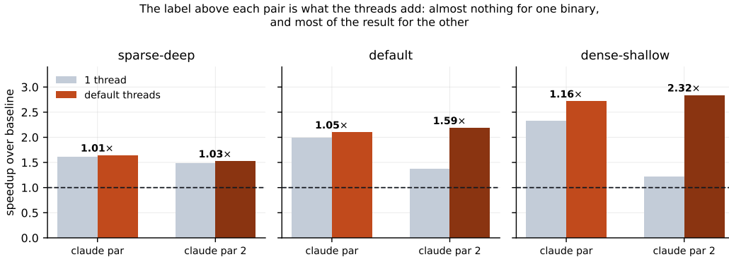
Figure 4: Each binary at one thread and at its own default, as speedup over baseline. The label above each pair is the default-thread mean divided by the one-thread mean — the part of the speedup that concurrency accounts for.
